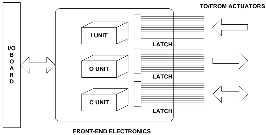
Fig. 5.5 - Actuator Control System layout for M1 active optics control
